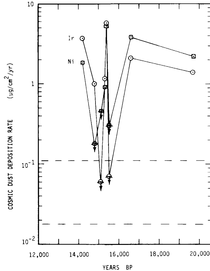
Fig. 4. Cosmic dust deposition rates recorded in the Camp Century ice core for the period 20000–14000 years BP. Curves marked Ir and Ni were respectively determined on the basis of measured iridium and nickel concentrations (LaViolette, 1985a).
