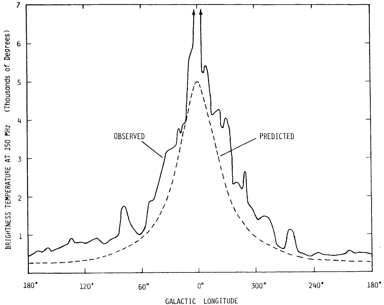
Fig. 11. Brightness temperature of the Galactic radio background emission as a function of galactic longitude. Solid line: the distribution observed at 150 MHz (after Price, 1974). Dashed line: the distribution predicted by the superwave model.
