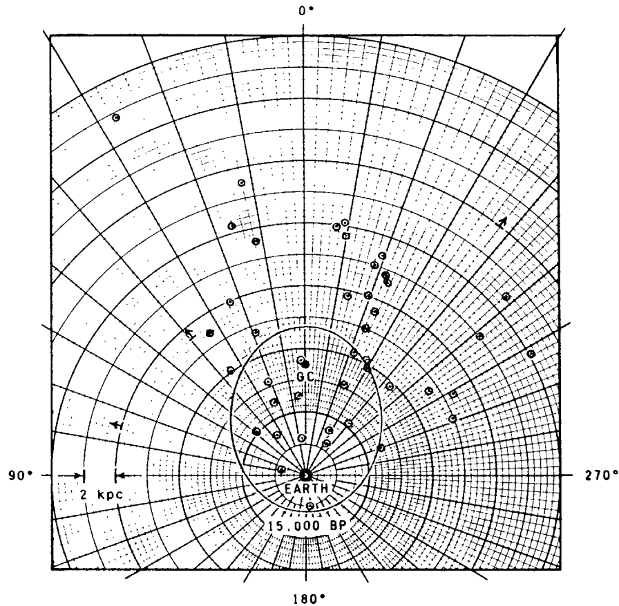
Fig. 14. The 15000 Year BP Superwave Event Horizon compared with the approximate locations of 46 medium surface brightness supernova remnants ( 0.1 < \Sigma < 1.0 f.u./(') 2 ).
